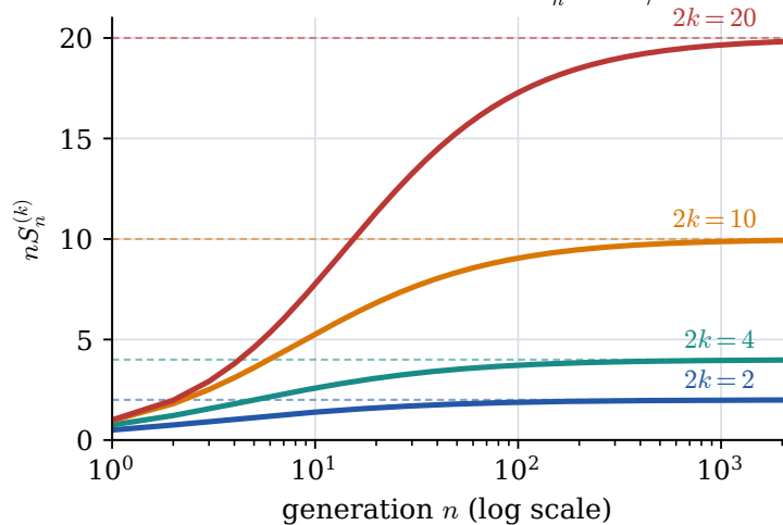
Common critical tail: S_n^{(k)} \sim 2k/n
